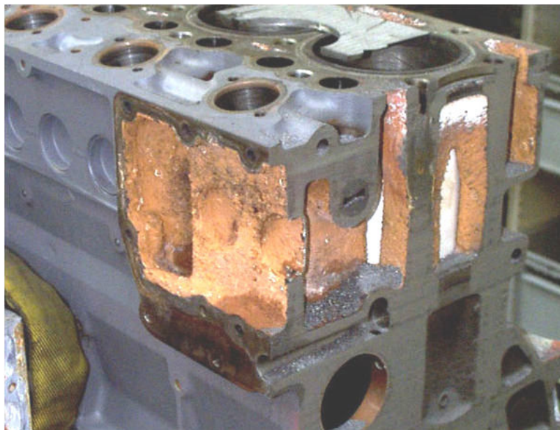
A 1 Crankcase
